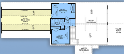
level two
