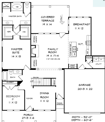
MAIN LEVEL FLOOR PLAN
