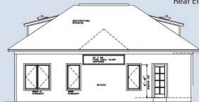
Rear Elevation
