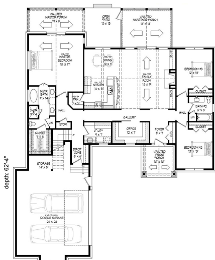
width: 72'-4" MAIN LEVEL FLOOR PLAN
