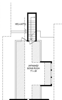
SECOND LEVEL FLOOR PLAN
